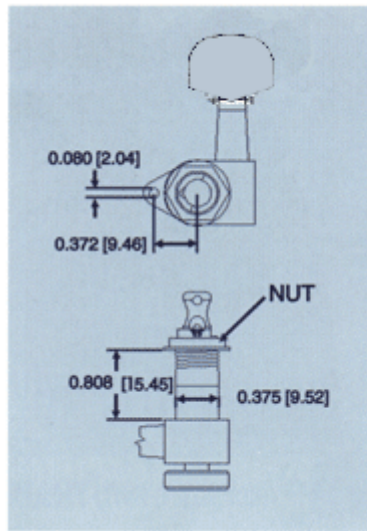
In-Line Auto Trim Dimensional Specs
