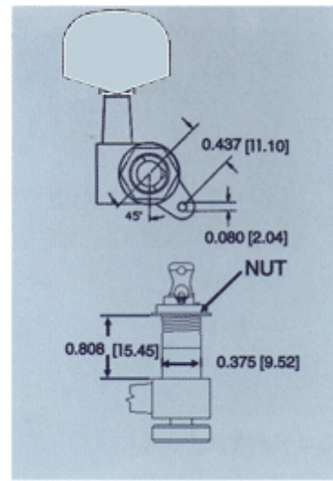
3+3 Auto Trim Dimensional Specs
